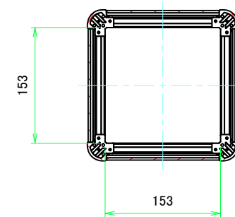
C-C (1:5)
